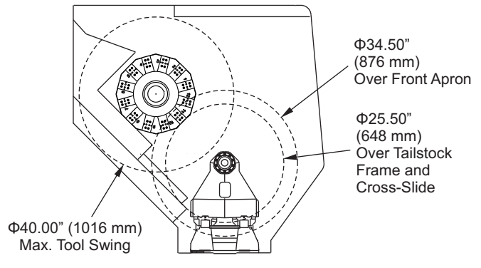
ST-40/45 Tool Swing Envelope Turret at Home Position 12-Station BOT Turret Standard
