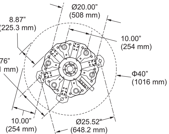
12-Station Hybrid VB12 Turret Option
