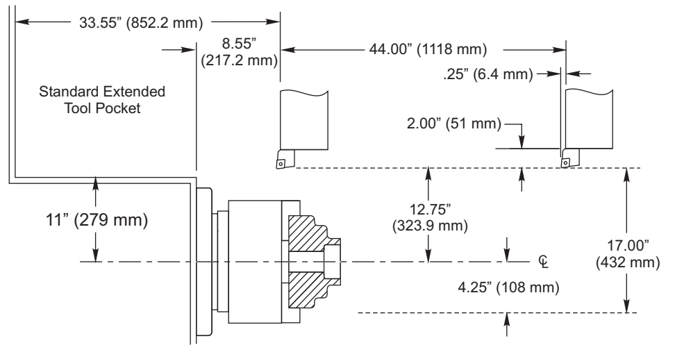
Axis Travels - ST-40/45 with Standard BOT
