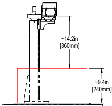
F290 F-THETA LENS MAX PART HEIGHT
