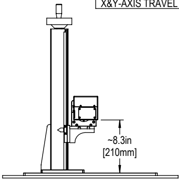
F160 F-THETA LENS HEIGHT
