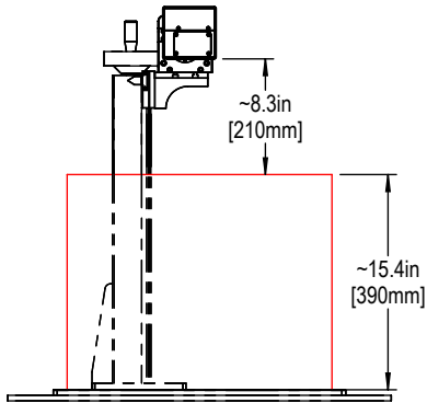
F160 F-THETA LENS MAX PART HEIGHT
