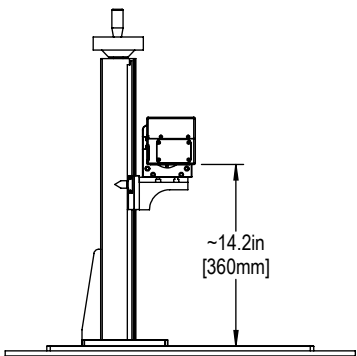
F290 F-THETA LENS HEIGHT
