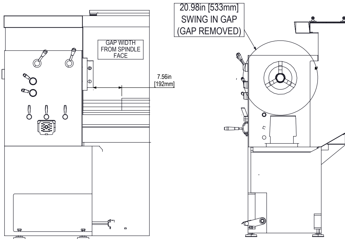
MAXIMUM SWING WITH GAP CASTING REMOVED
