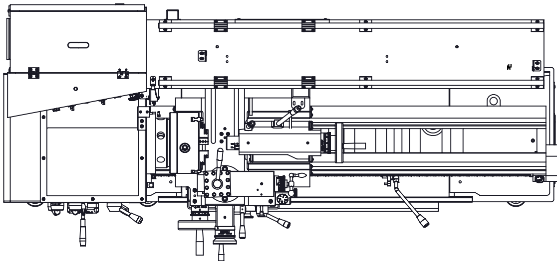
CARRIAGE, CROSS SLIDE AND TAILSTOCK NEAR THE CHUCK
