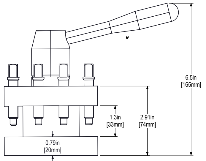
4-STATION MANUAL TOOL POST FOR 20mm (0.787in) TOOLS
