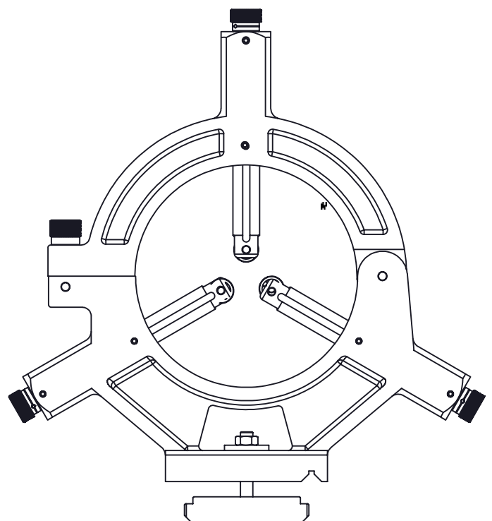
STEADY MINIMUM \varnothing 1.5in [ \varnothing 38mm]
