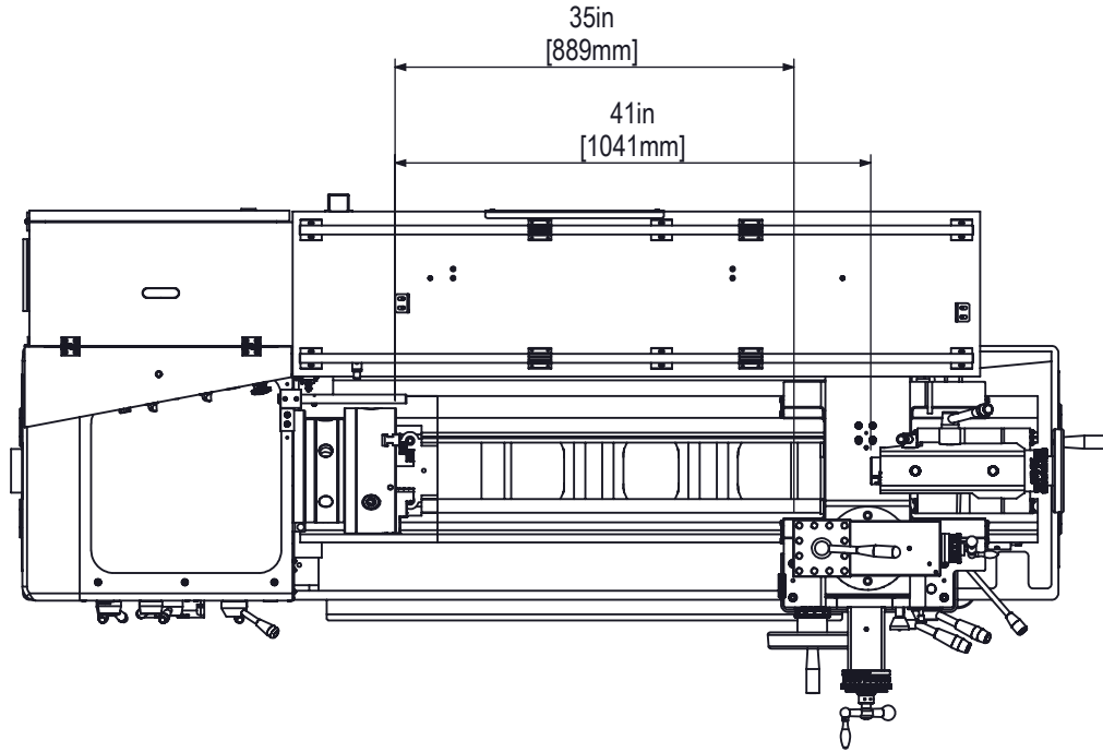
CARRIAGE, CROSS SLIDE AND TAILSTOCK AWAY FROM THE CHUCK
