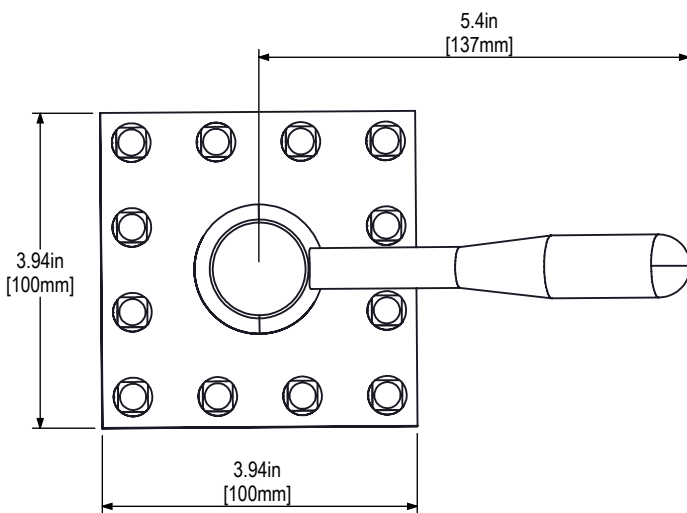
4-STATION MANUAL TOOL POST FOR 20mm (0.787in) TOOLS
