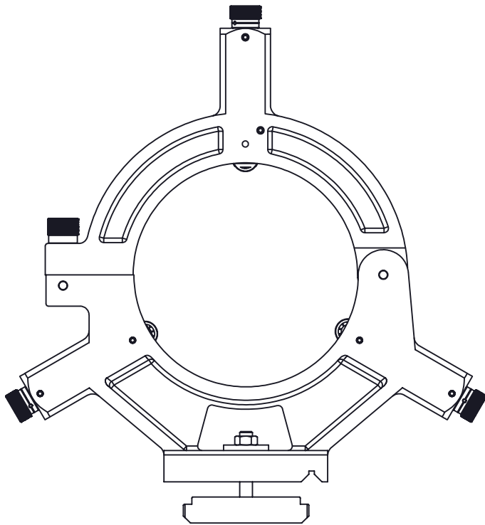
STEADY MAXIMUM \varnothing 8.27in [ \varnothing 210mm]
