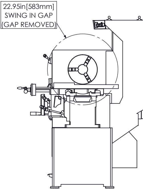
MAXIMUM SWING WITH GAP CASTING REMOVED
