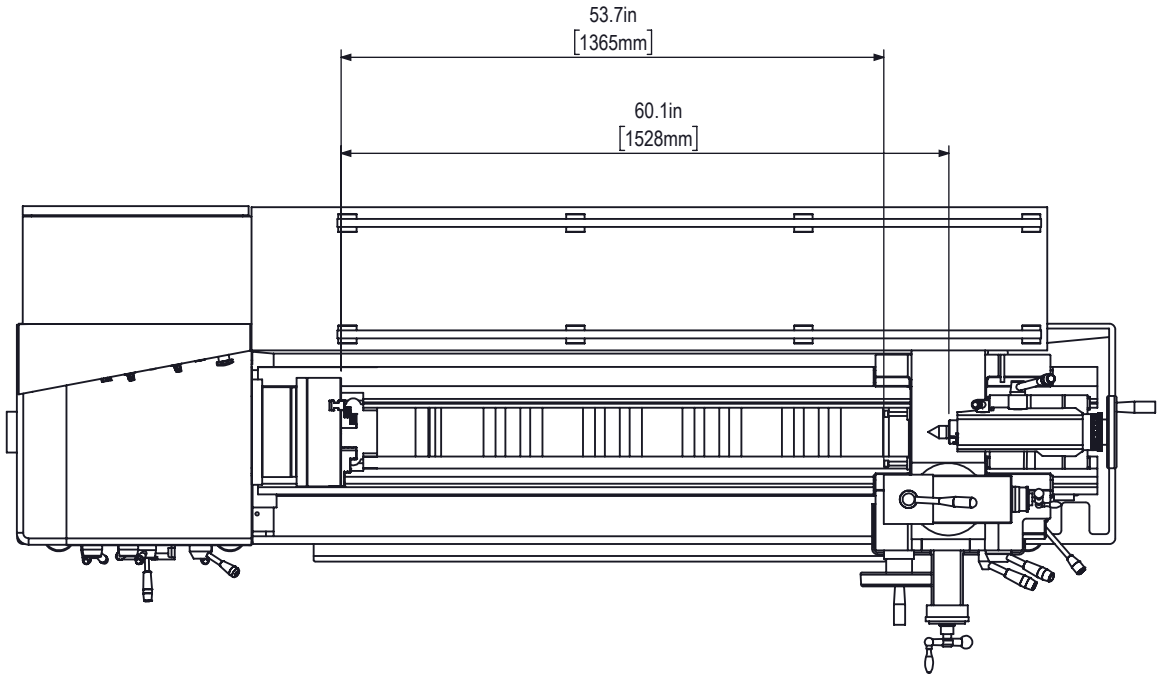
CARRIAGE, CROSS SLIDE AND TAILSTOCK AWAY FROM THE CHUCK
