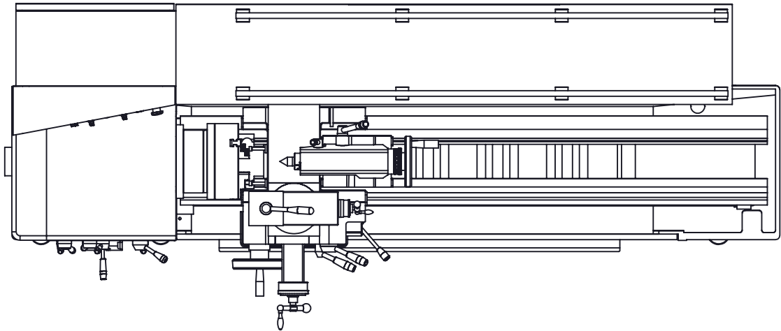
CARRIAGE, CROSS SLIDE AND TAILSTOCK NEAR THE CHUCK
