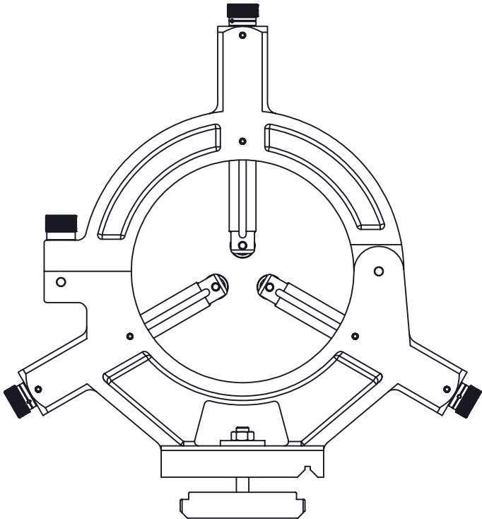
STEADY MINIMUM \phi 1.5\text{in} [38mm]
