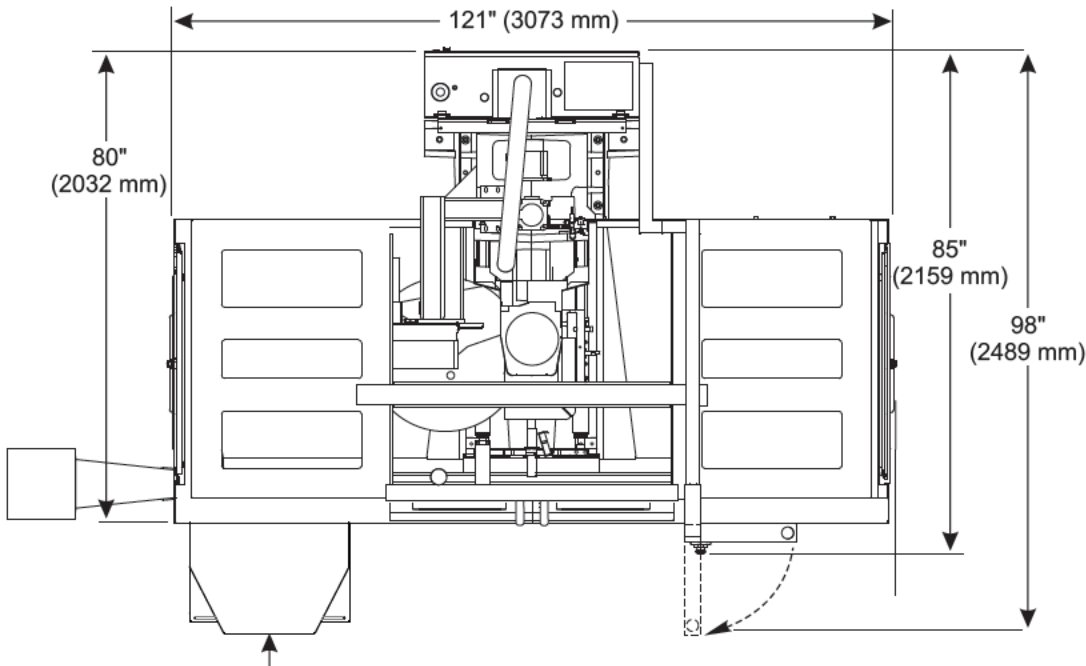
TM-3 Anchor Pattern
