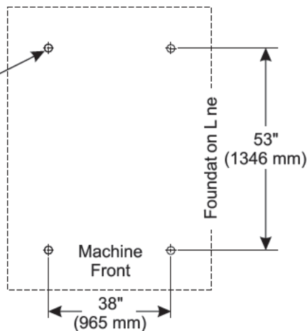
TM-3 Anchor Pattern
