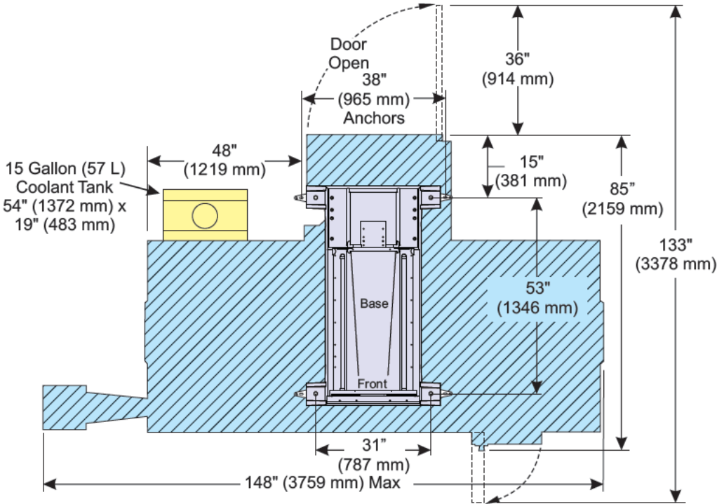
TM-3 Sheet Metal Removed for Clarity
