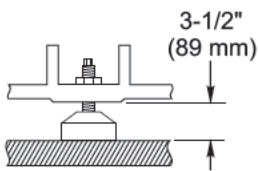
4X Leveling Pad Pin Dimension
