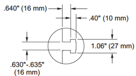
Detail B (5X)
