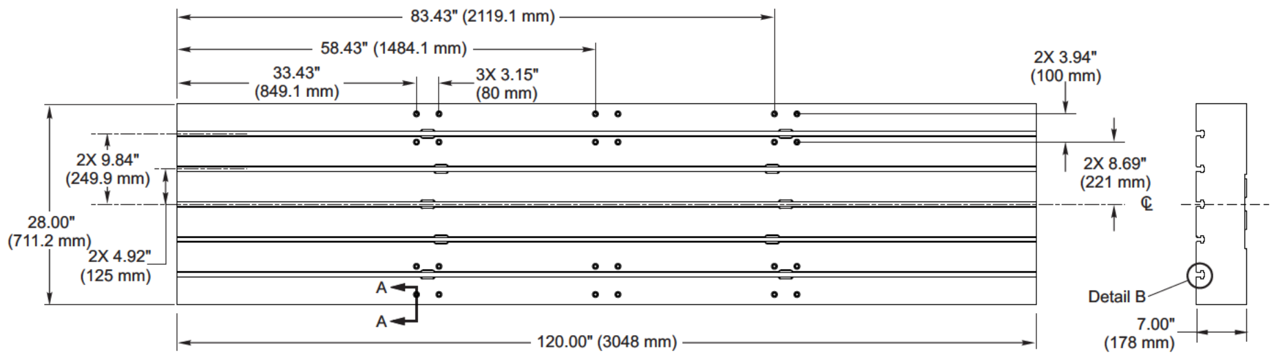
Front View
