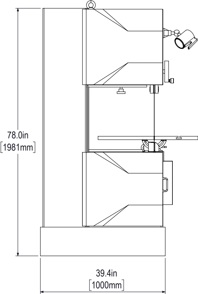
FRONT VIEW (OPERATOR)
