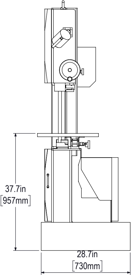
SIDE VIEW
